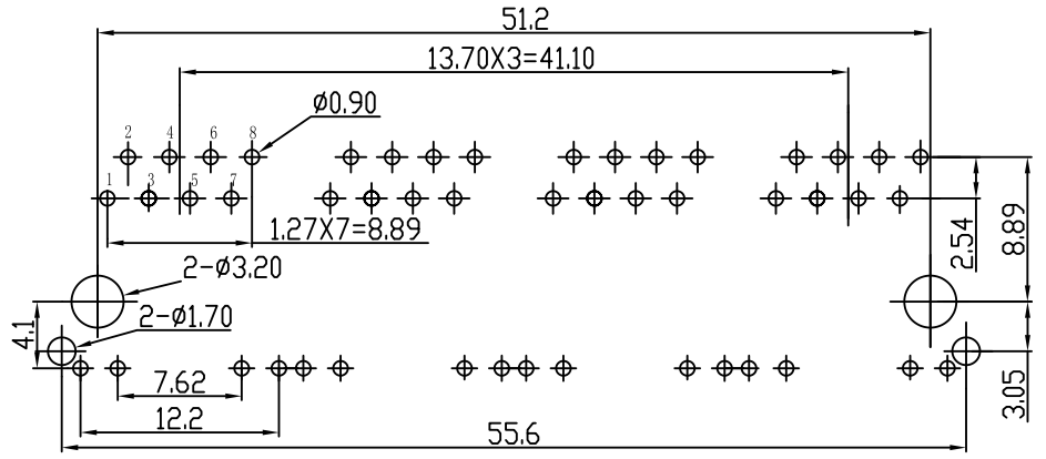
PC Board Layout H=1.6T
